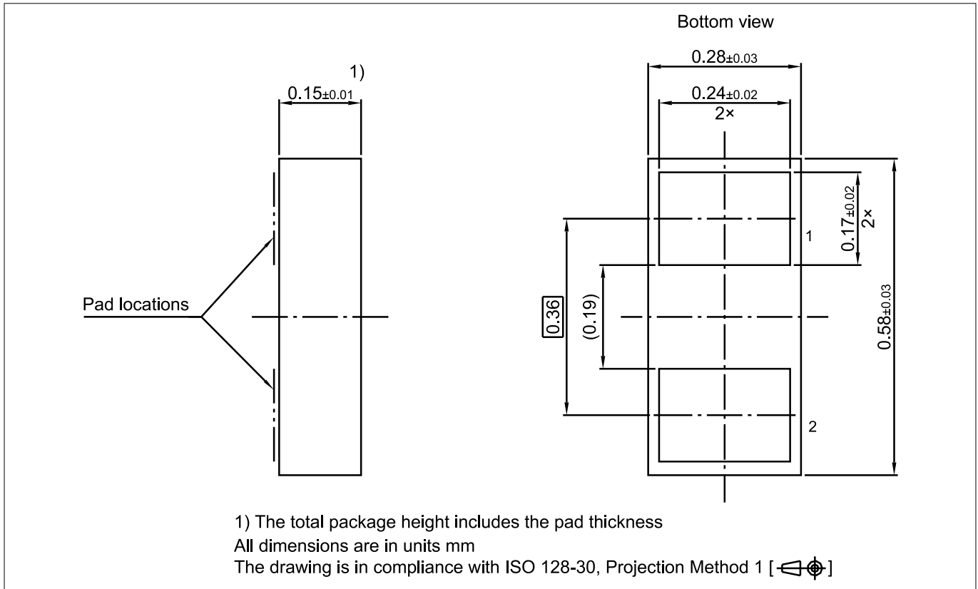
Figure 12 WLL-2-3 package
