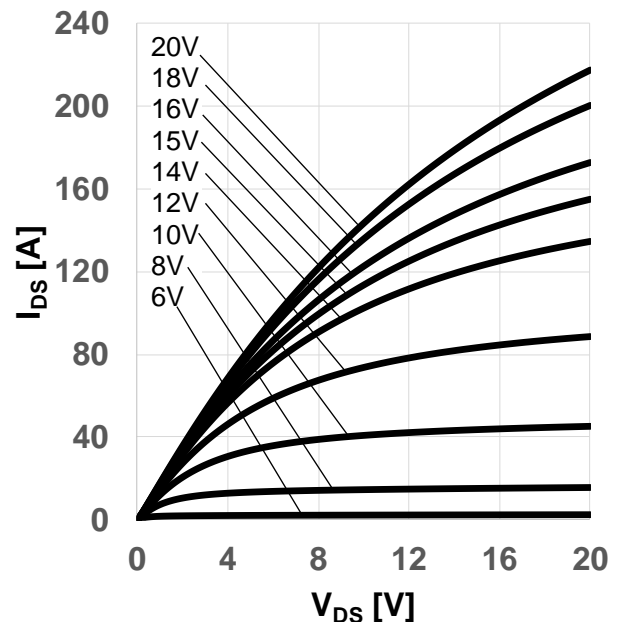
Figure 8 Typical output characteristic, V_{GS} as parameter ( I_{DS} = f(V_{DS}), T_{vj}=175°C, t_P = 20\mu s )
