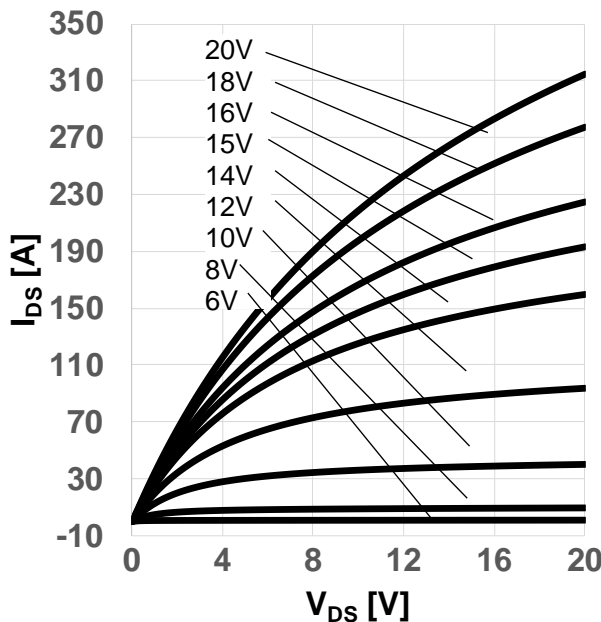
Figure 7 Typical output characteristic, V_{GS} as parameter ( I_{DS} = f(V_{DS}), T_{vj}=25°C, t_P = 20\mu s )
