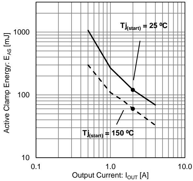
Figure 23. Active Clamp Energy vs Output Current
