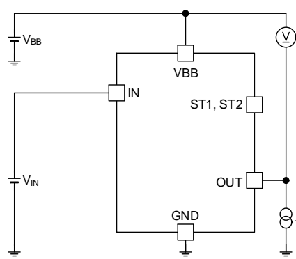
Figure 27. Output ON Resistance Output Clamp Voltage
