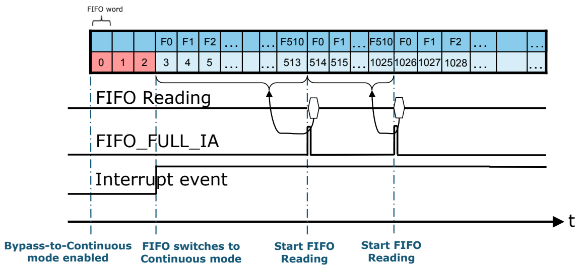
Figure 10. Bypass-to-continuous mode
