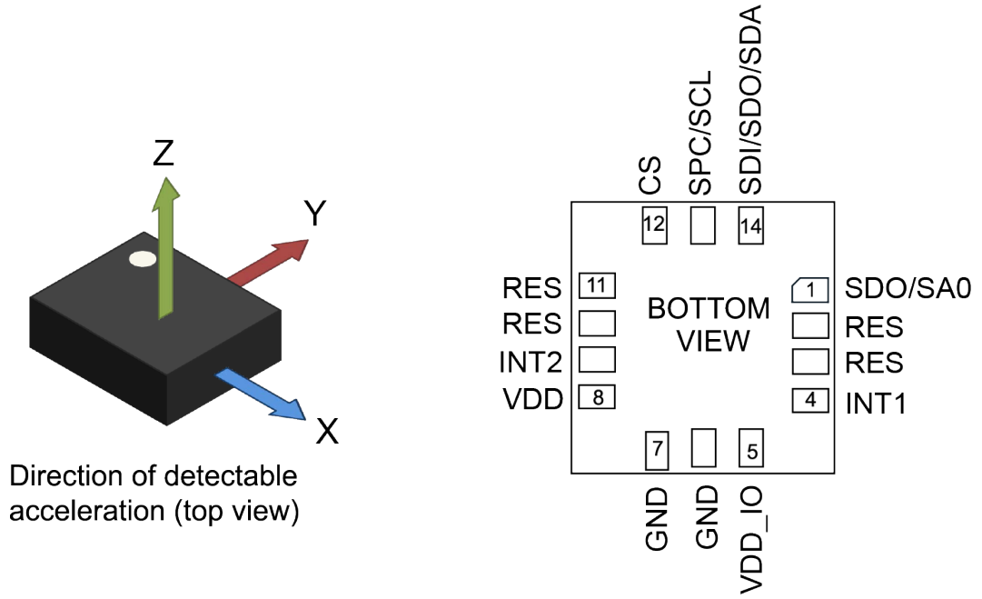
Figure 1. Pin connections
