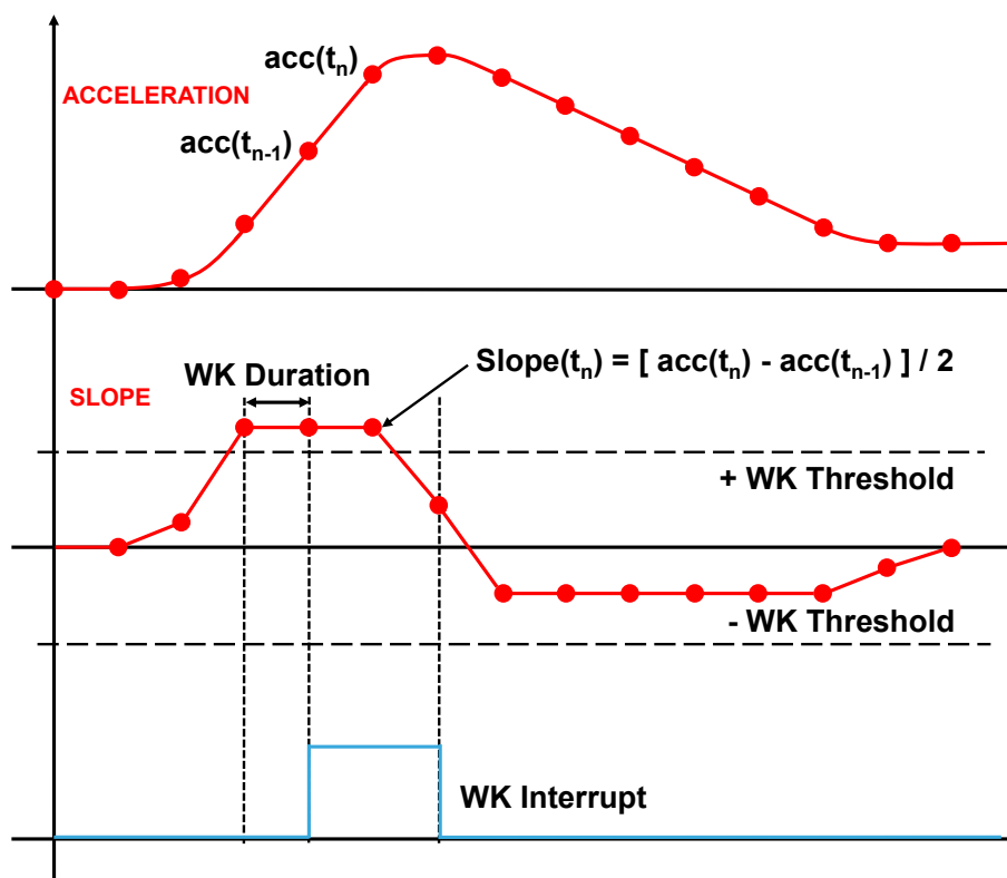
Figure 5. Wake-up interrupt (using the slope filter)
